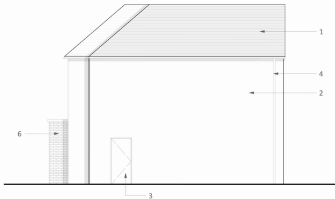
2 Proposed East Elevation Scale: 1:100
