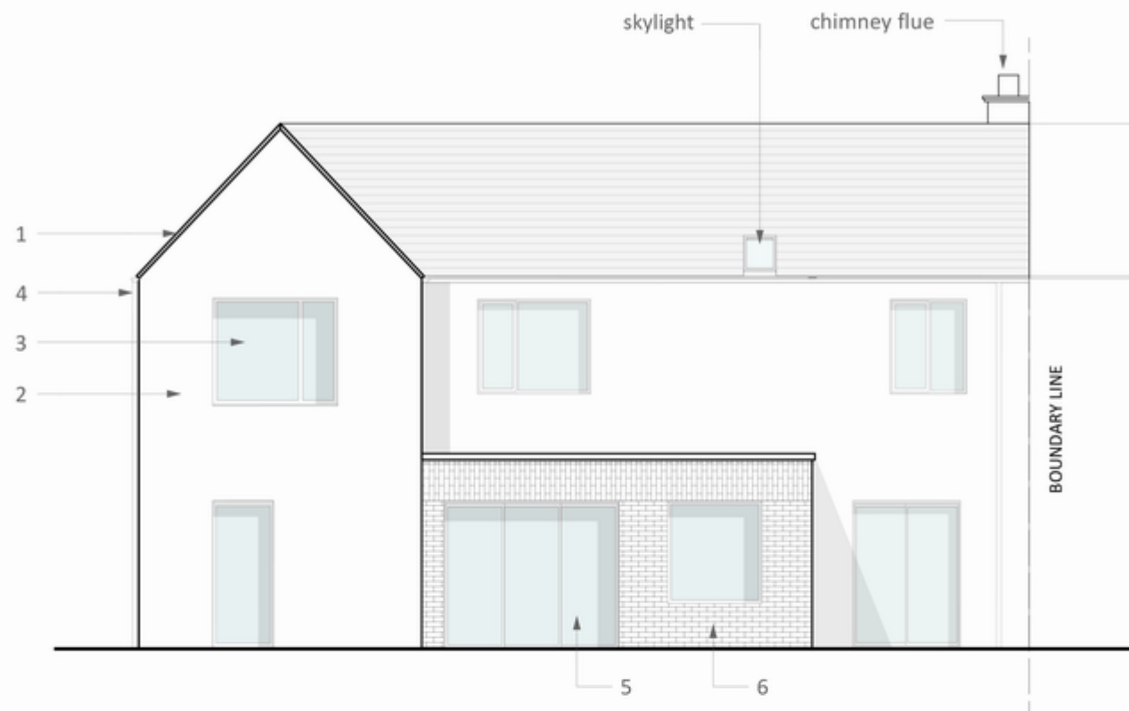
1 Proposed North Elevation Scale: 1:100
