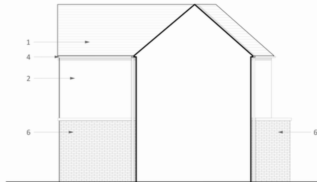
4 Proposed West Elevation Scale: 1:100
